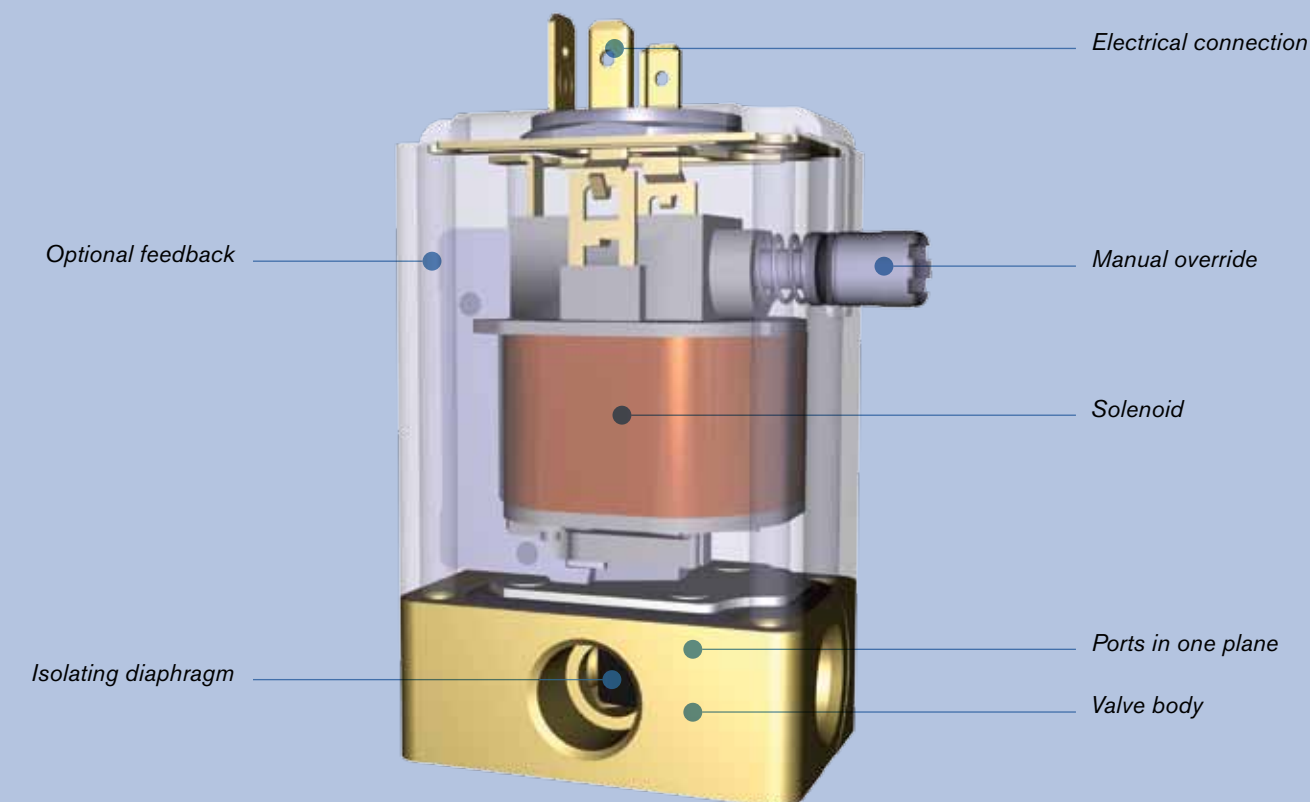
Pivoted armature valve type 0330
