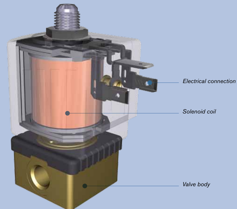
3/2-way plunger-type solenoid valve type 6014
