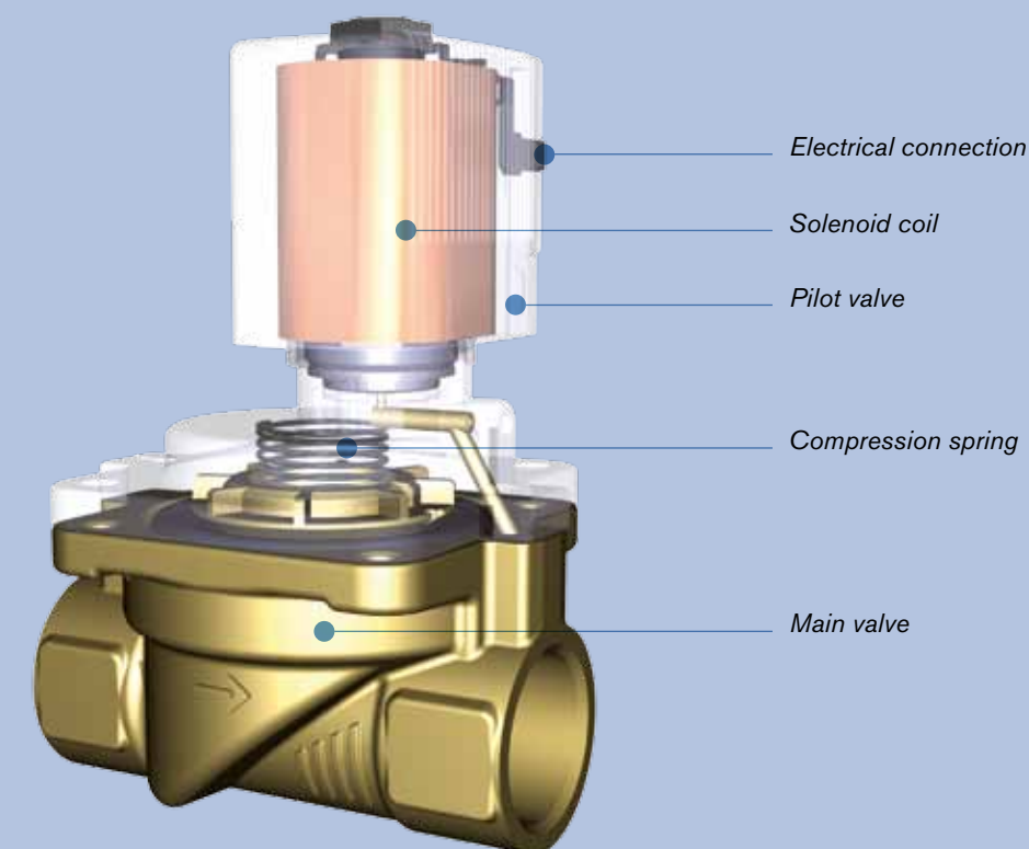
Servo assisted solenoid valve with diaphragm type 5281
