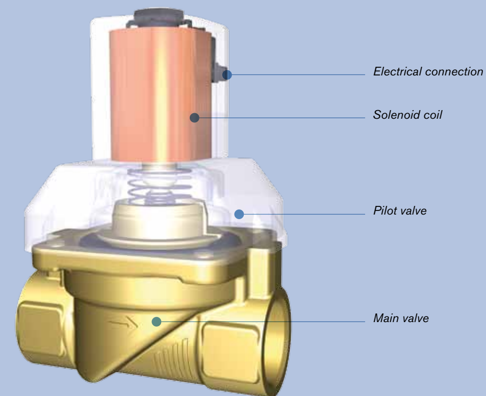
2/2-way spring coupled servo assisted solenoid valve type 6213
